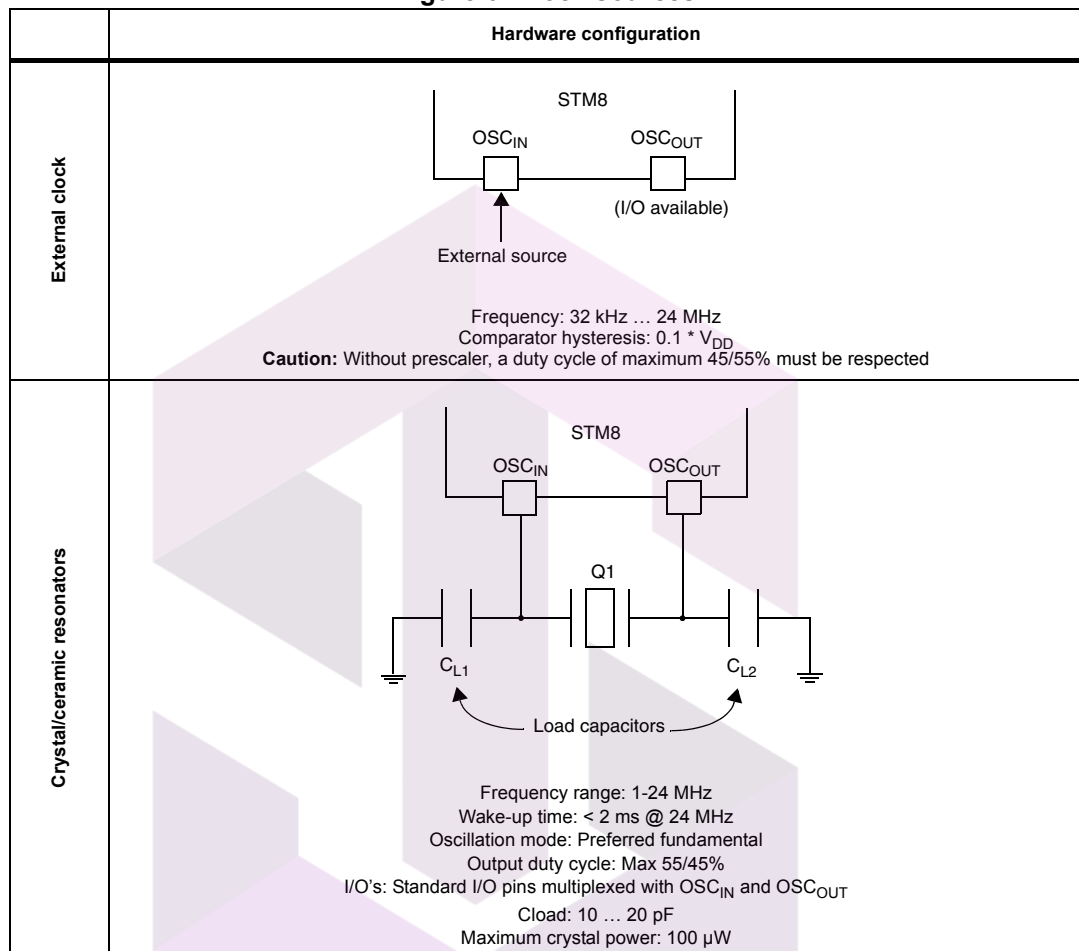
Figure 6. Clock sources
