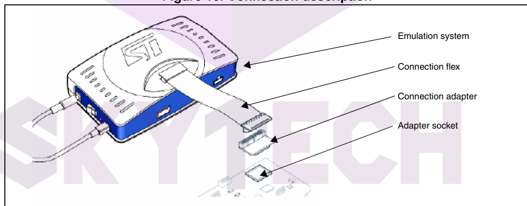
Figure 13. Connection description
