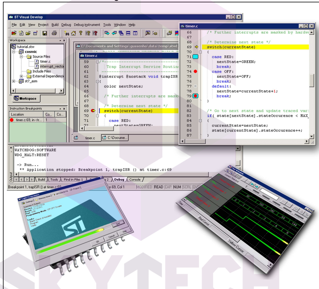
Figure 16. Software toolchain
